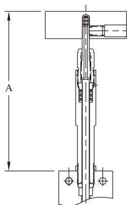
Cylindrical Bonnet
