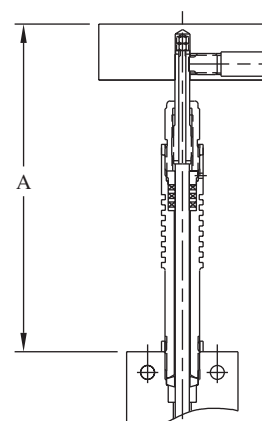
Finned Bonnet
